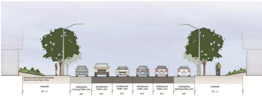
Masonic Avenue Typical Existing Roadway Section
