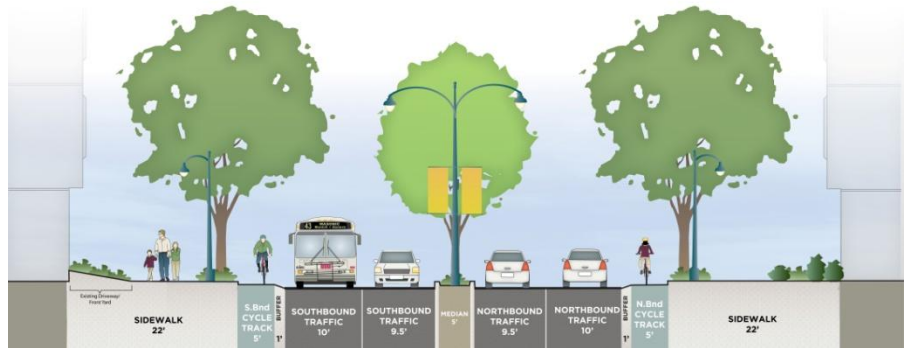
Masonic Avenue Typical Proposed Roadway Section
