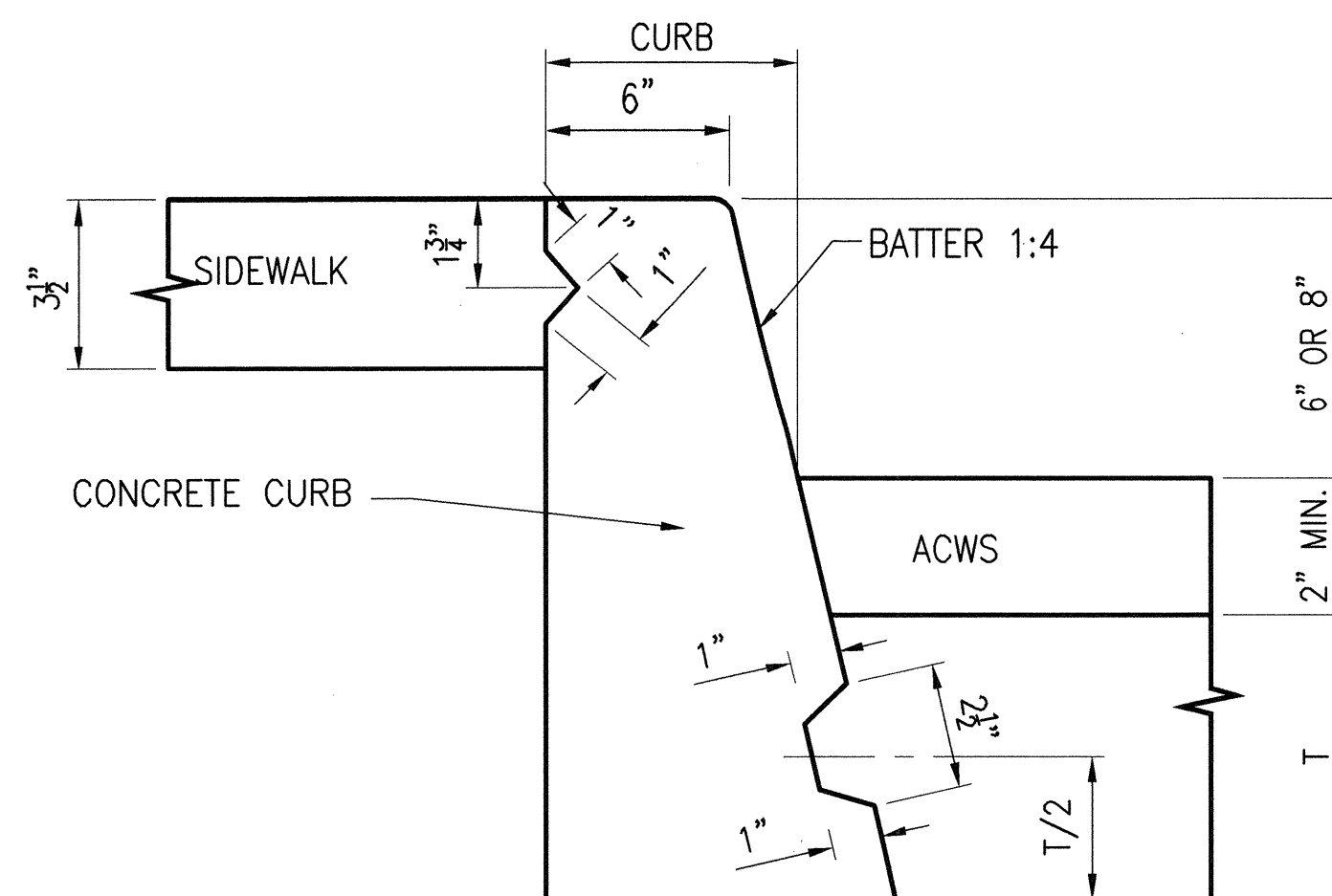
LONGITUDINAL CONSTRUCTION JOINTS FOR CONCRETE CURB
