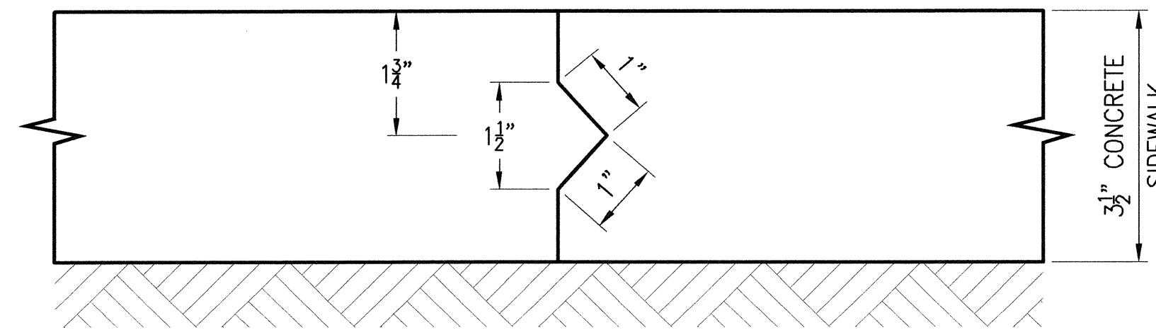
TRANSVERSE CONSTRUCTION JOINT FOR CONCRETE SIDEWALK
