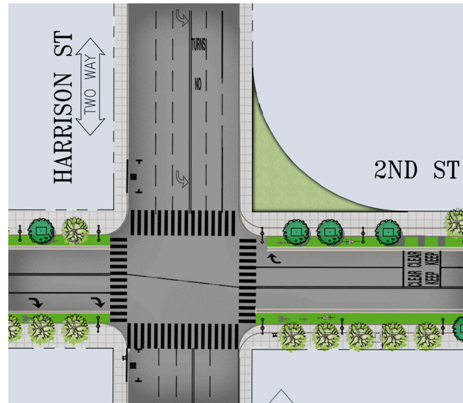
REMOVAL OF DUAL RIGHT TURN AT HARRISON AND PAVEMENTS TO PARK SITE
