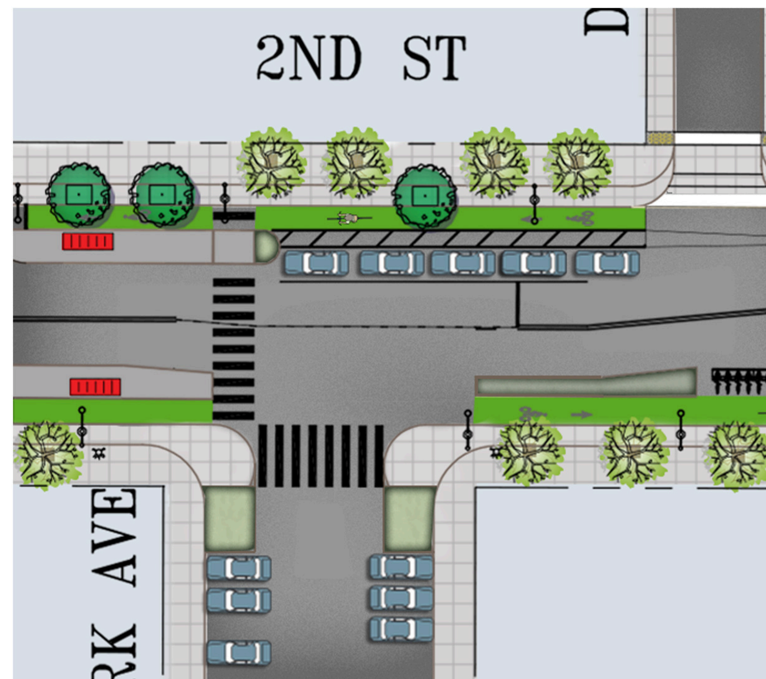
ENHANCED BULB-OUTS AND NEW TRAFFIC SIGNAL AT SOUTH PARK ENTRANCE
