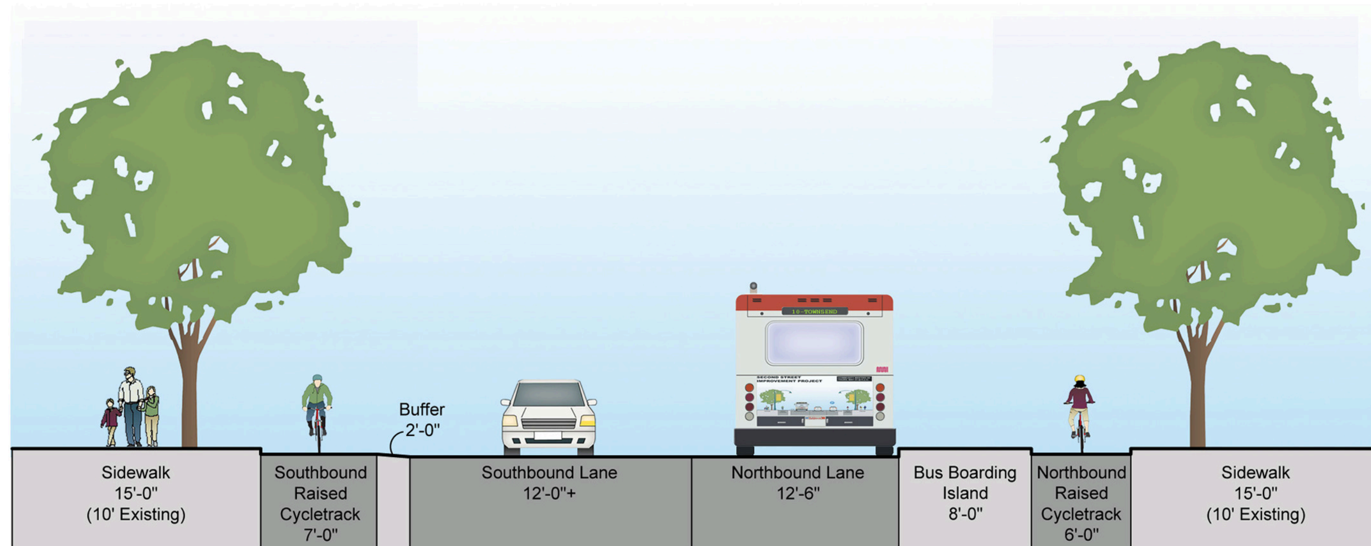
TYPICAL SECTION AT BUS BOARDING ISLANDS
