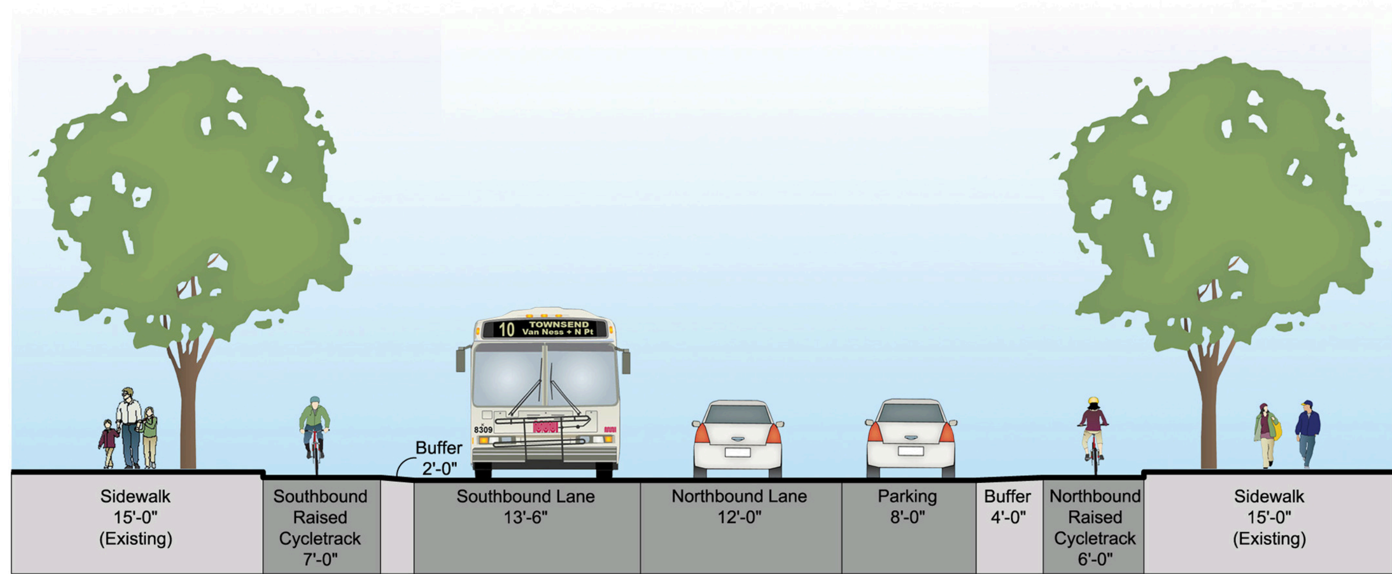
MARKET STREET TO HARRISON STREET
