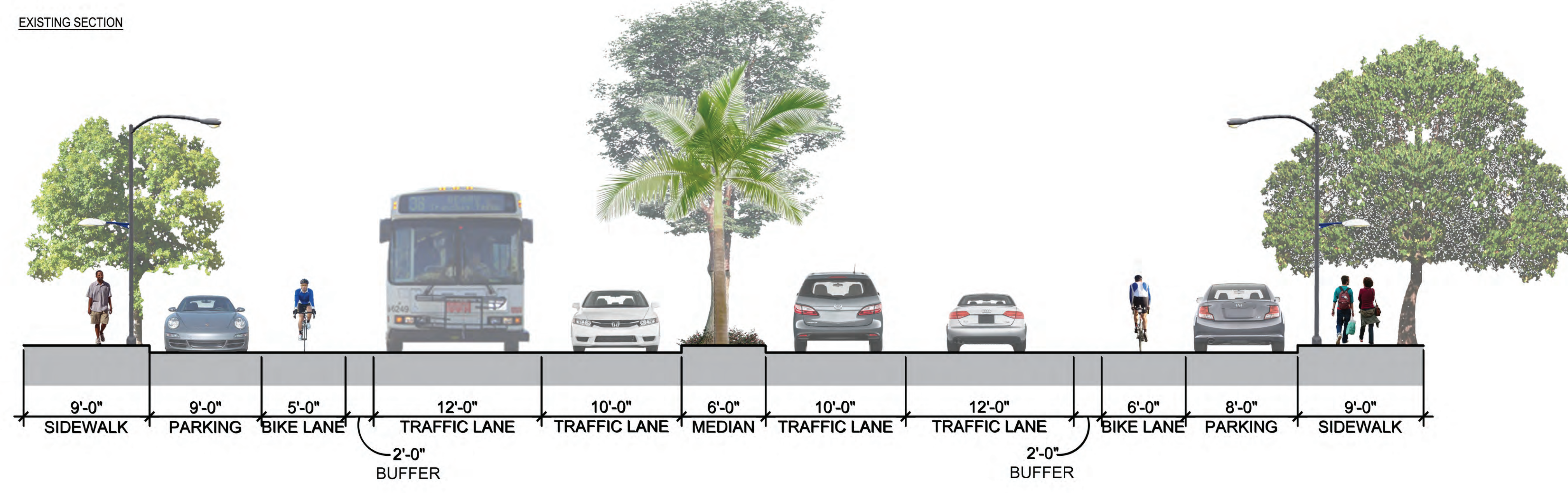
PROPOSED SECTION B-B
