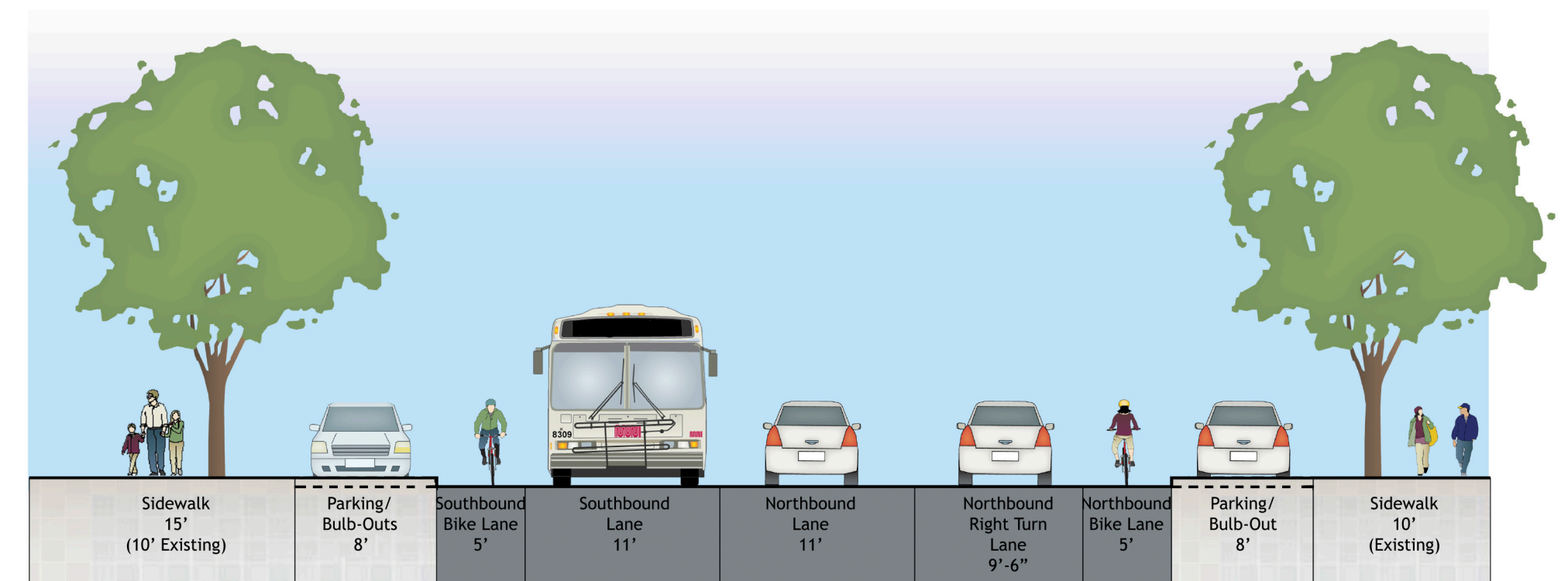
Bike Lanes Bryant to Townsend Bike Lanes, Parking Both Sides, Bulb-Outs, Optional Turn Lane
