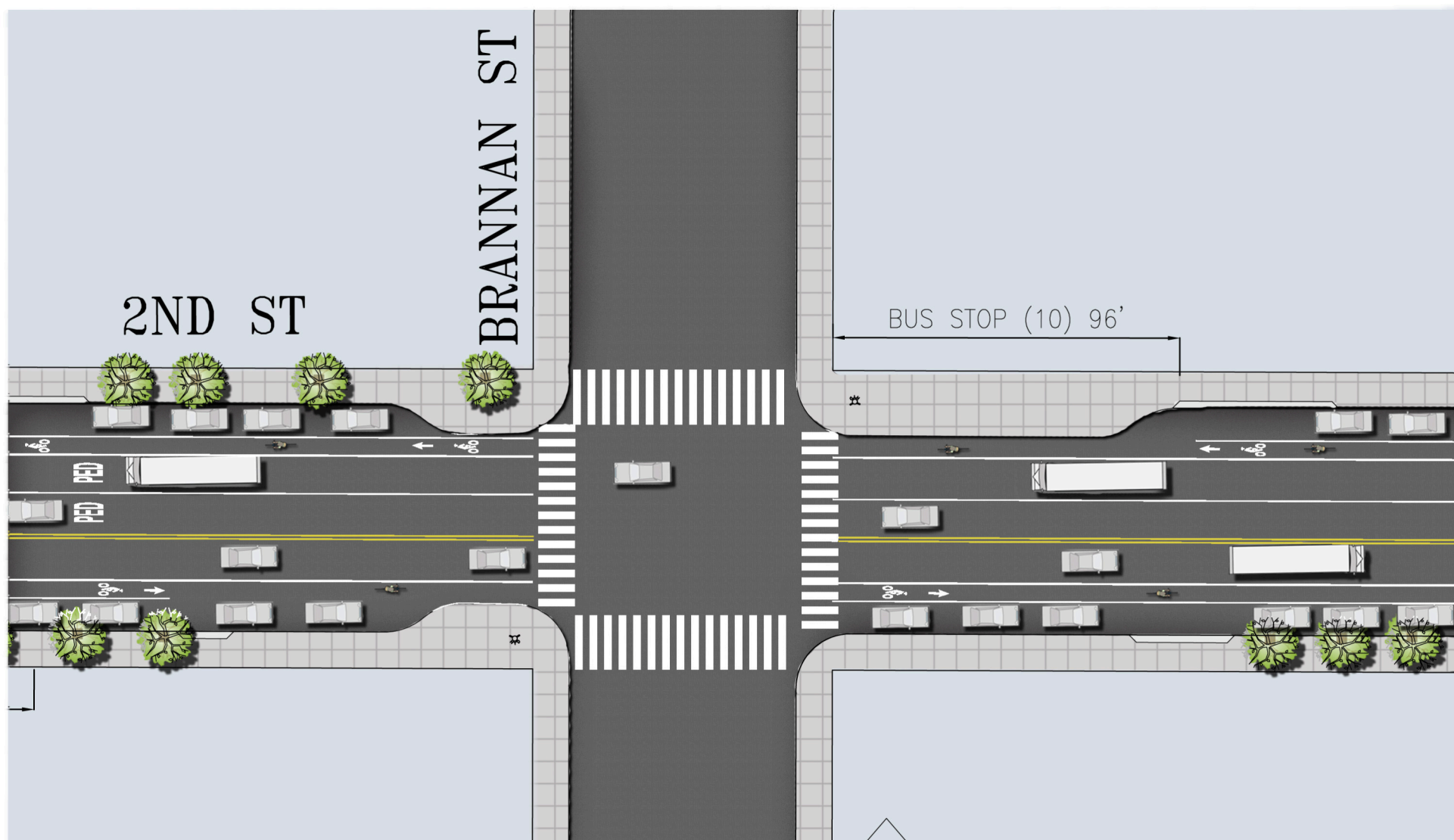
CONCEPTUAL PLAN VIEW OF A TYPICAL INTERSECTION: 2ND STREET AT BRANNAN STREET
