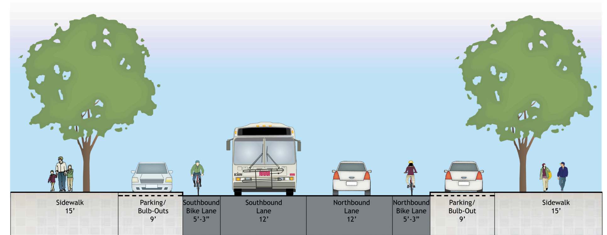
Bike Lanes Market to Harrison Bike Lanes, Parking Both Sides, Bulb-Outs
