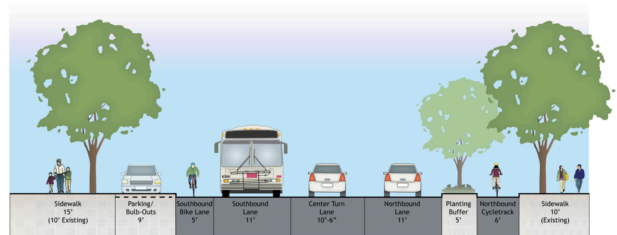
Center Turn Lanes Bryant to Townsend Center Turn Lanes, Bulb-Outs, Cycletrack East Side, Bike Lane, Parking West Side
