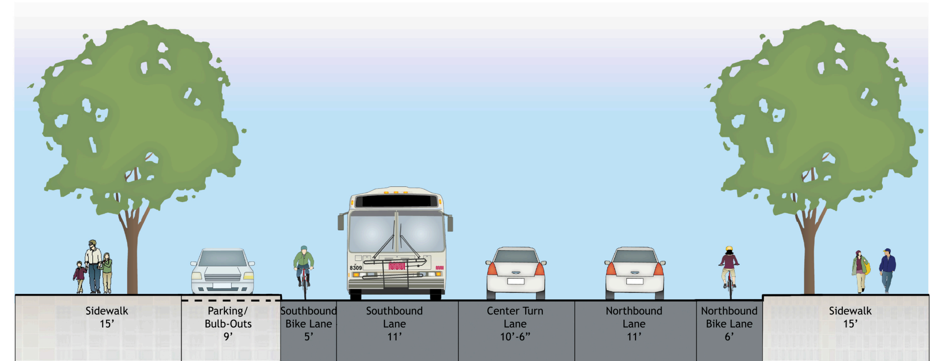
Center Turn Lanes Market to Harrison Center Turn Lanes, Bulb-Outs, Cyclercrack East Side, Bike Lane, Parking West Side
