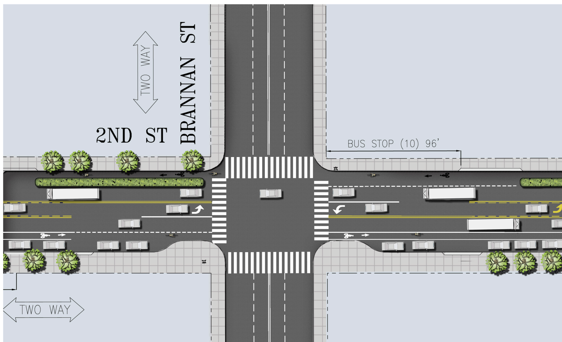
CONCEPTUAL PLAN VIEW OF A TYPICAL INTERSECTION: 2ND STREET AT BRANNAN STREET
